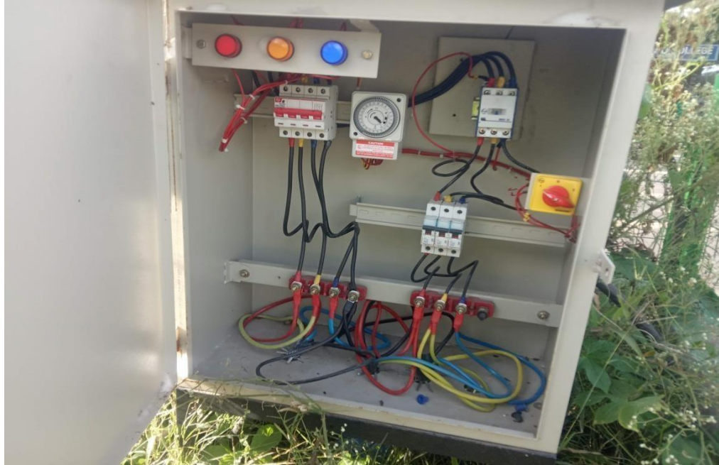
Butterfly Light Automatic Switch On/Off System
