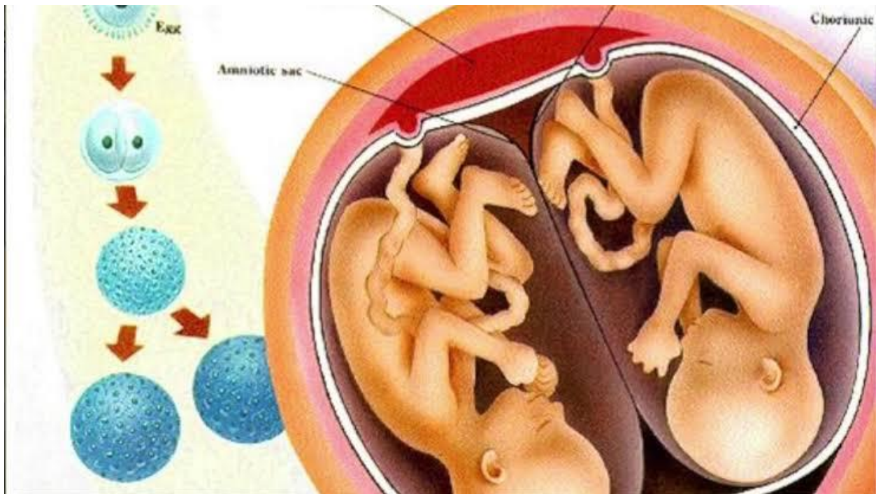
IDENTICAL TWINS
