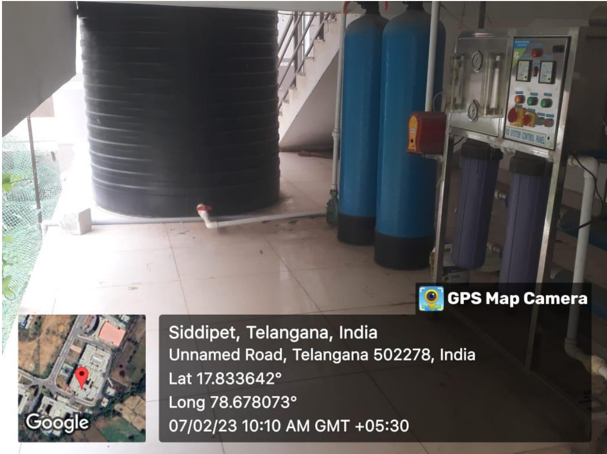
R.O Plant
