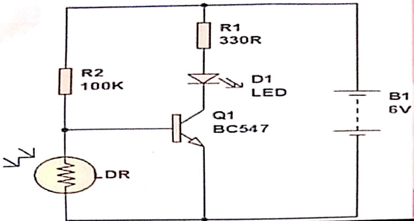
Figure - Circuit diagram of automatic street light controller
