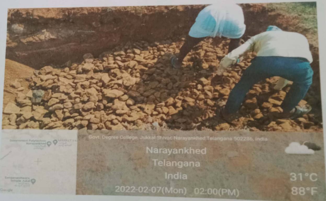
Covering of the Pit with Stones
