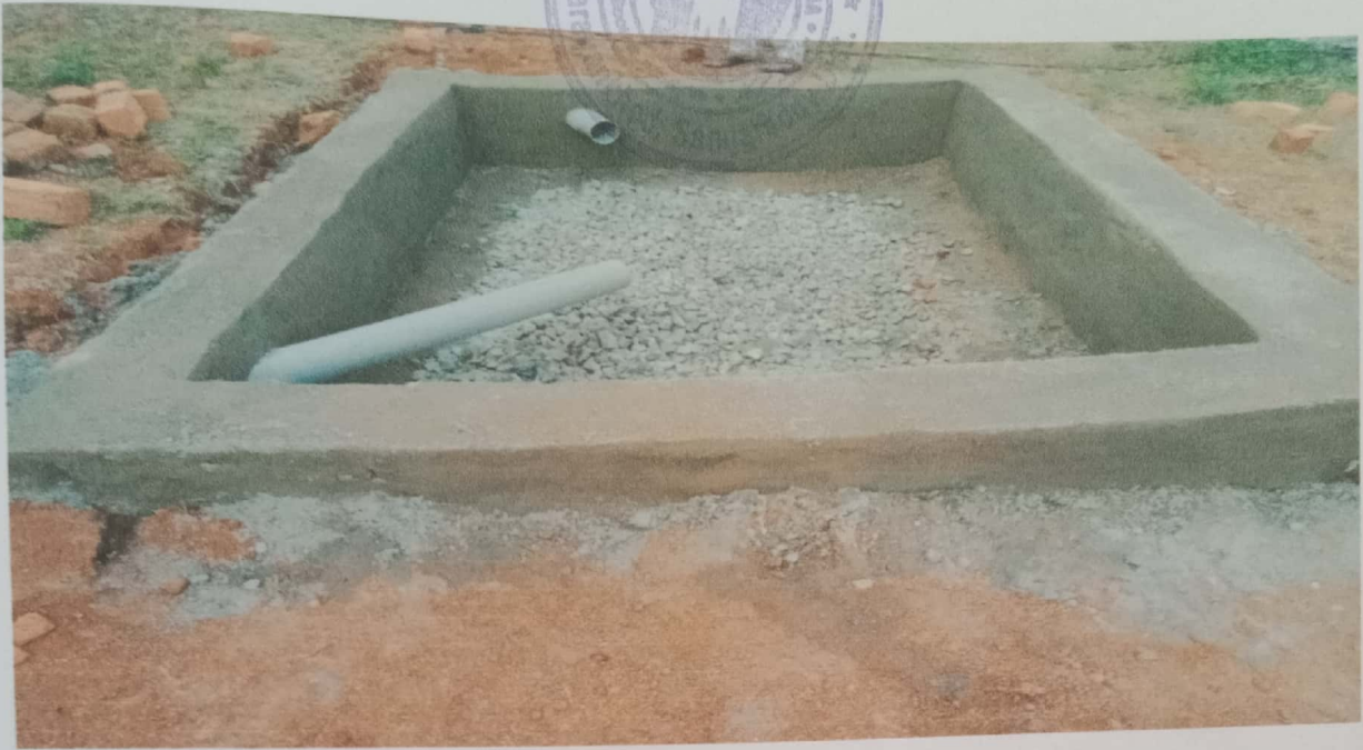
Final Stage of Rain Harvesting Pit - 1
