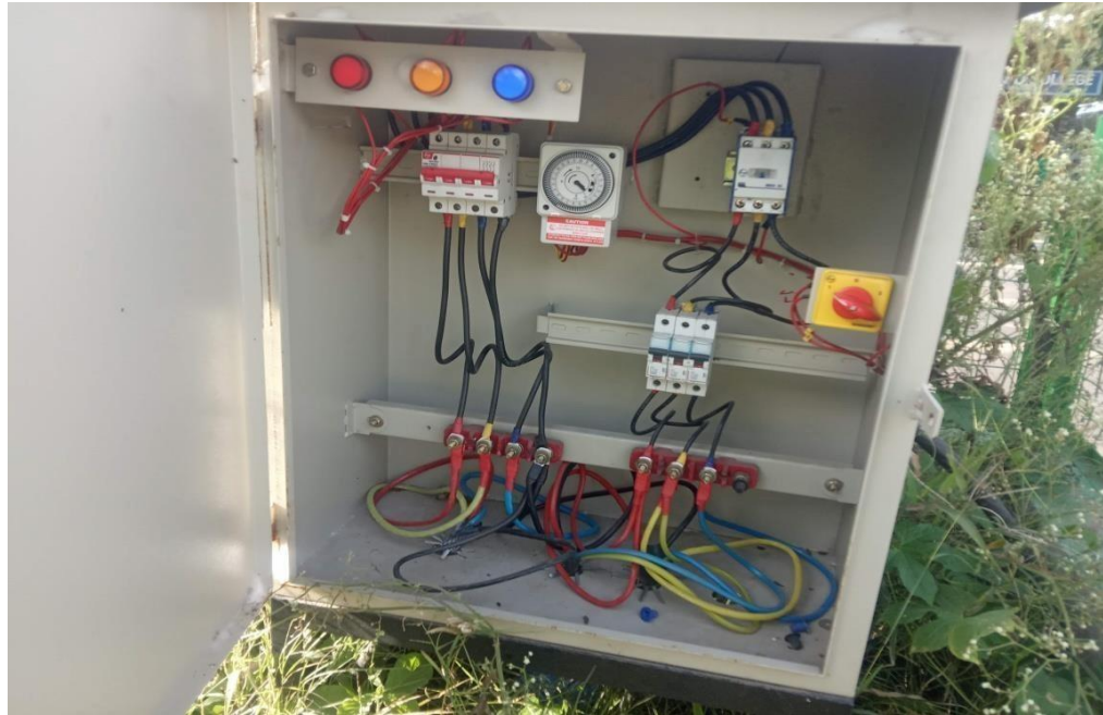
Butterfly Light Automatic Switch On/Off System
