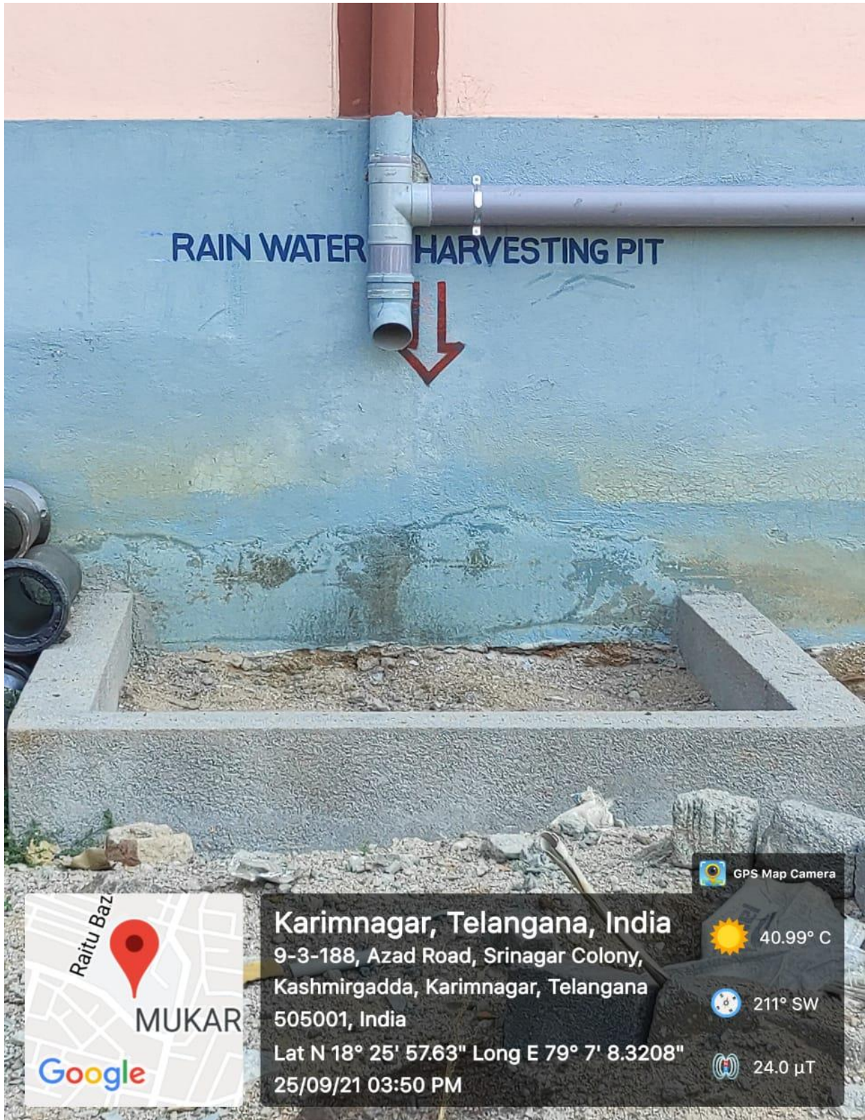
Rain water harvesting pit 03
