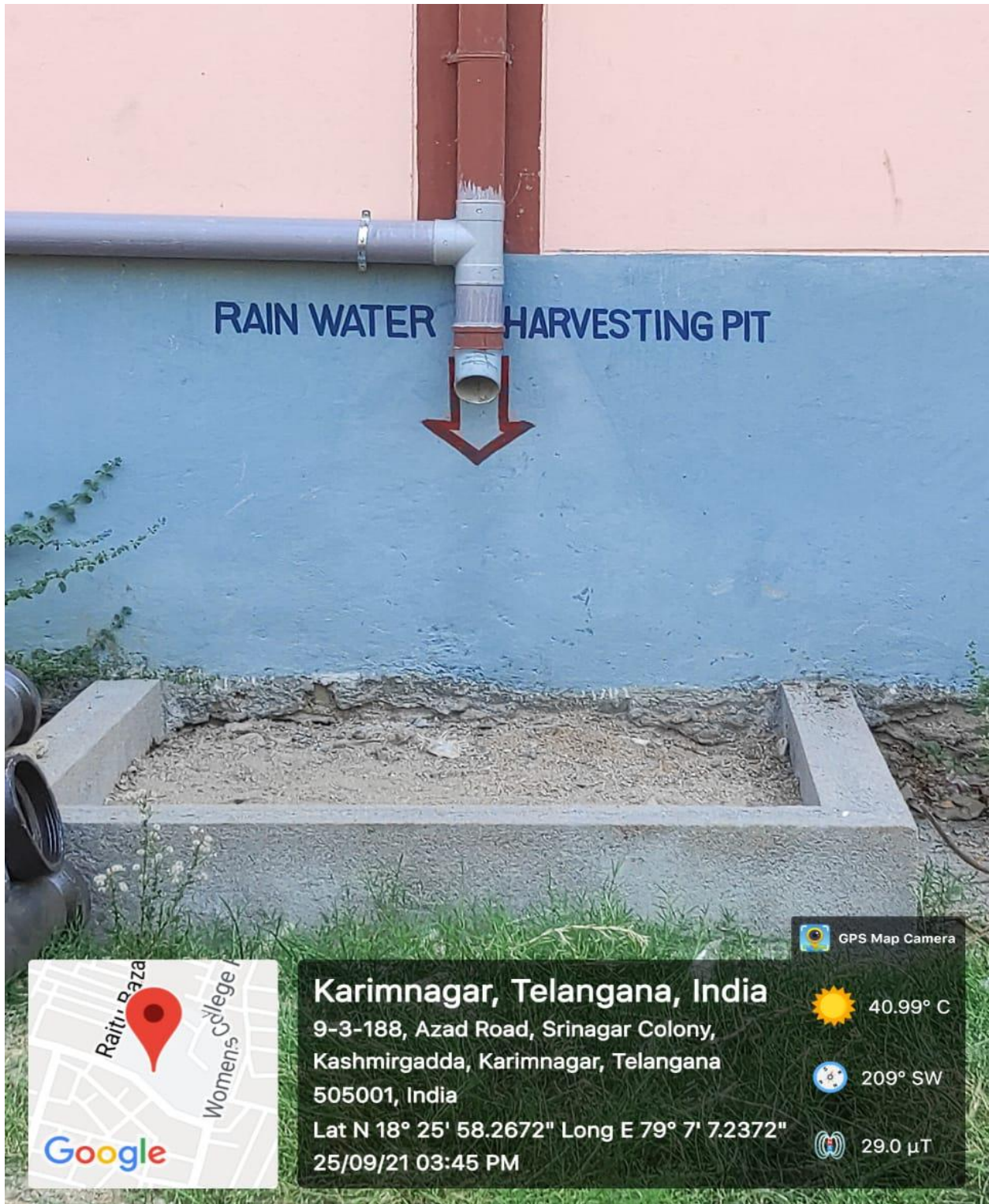
Rain water harvesting pit 02
